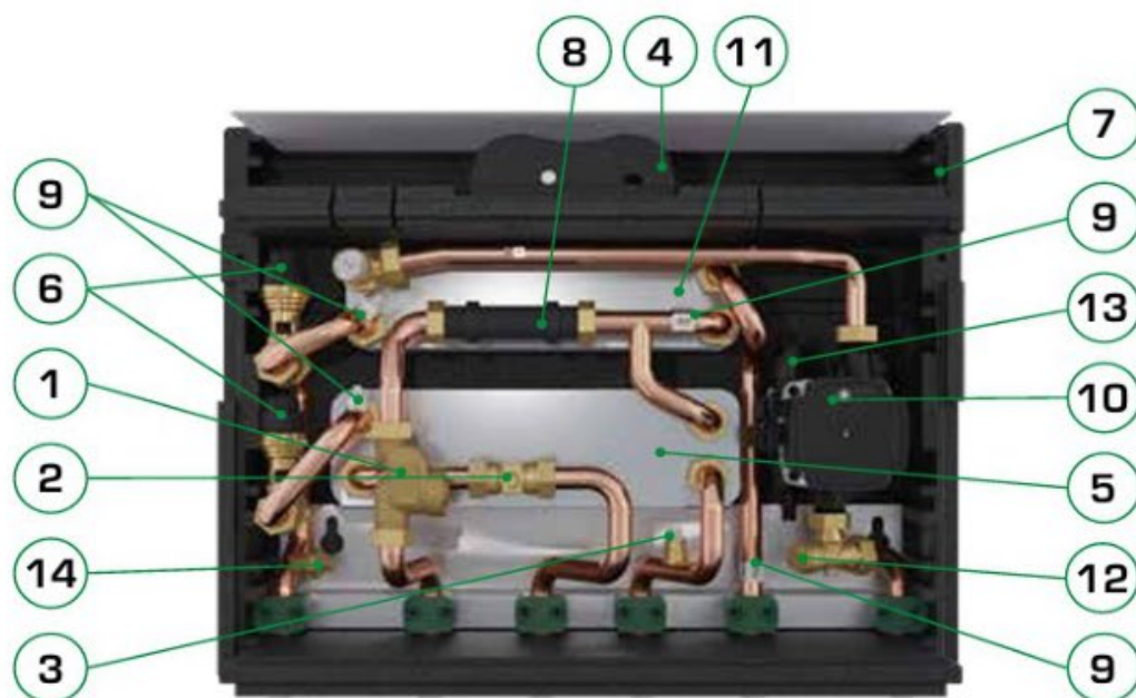
Exploded view AquaHeat HEX-140
